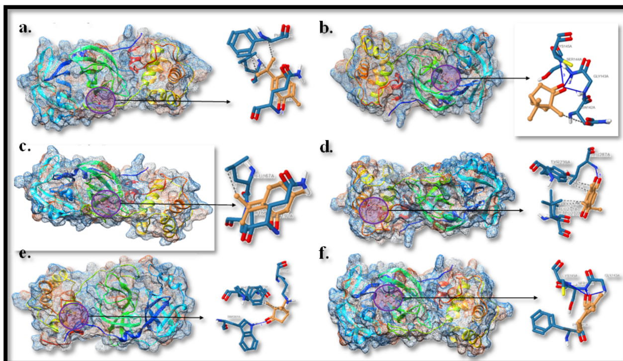
Figure 3. Binding site for ligands in protease of hosts. The active site has been highlighted, surface and cartoon representation in a black box and the cavity has been magnified to display the residues in each case. Distinct bond distance along with bond between hetero atoms and other atoms is also shown in a mess structure. Here (a) 2gtb-Thymoquinone, (b) 2gtb-Camphor, (c) 2gtb-Pulegone, (d) 6lu7-Thymoquinone, (e) 6lu7-Camphor, and (f) 6lu7-Pulegone.
