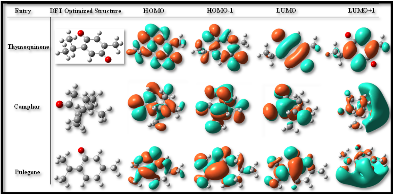
Figure 5. Electron density maps of HOMO and LUMO of keto-based ligands through DFT calculation.
