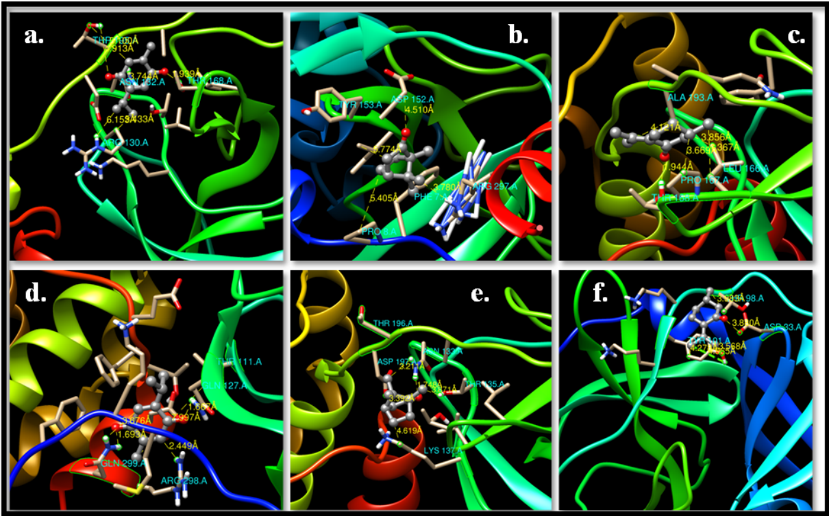
Figure 4. Binding site detection using CCDC Gold programme. Specific bond distances along with atom name and hetero atoms are displayed for each case i.e., (a) 2gtb- Thymoquinone, (b) 2gtb- Camphor, (c) 2gtb-Pulegone, (d) 6lu7-Thymoquinone, (e) 6lu7-Camphor, and (f) 6lu7-Pulegone. The smallest bond distance shows the good binding site.
