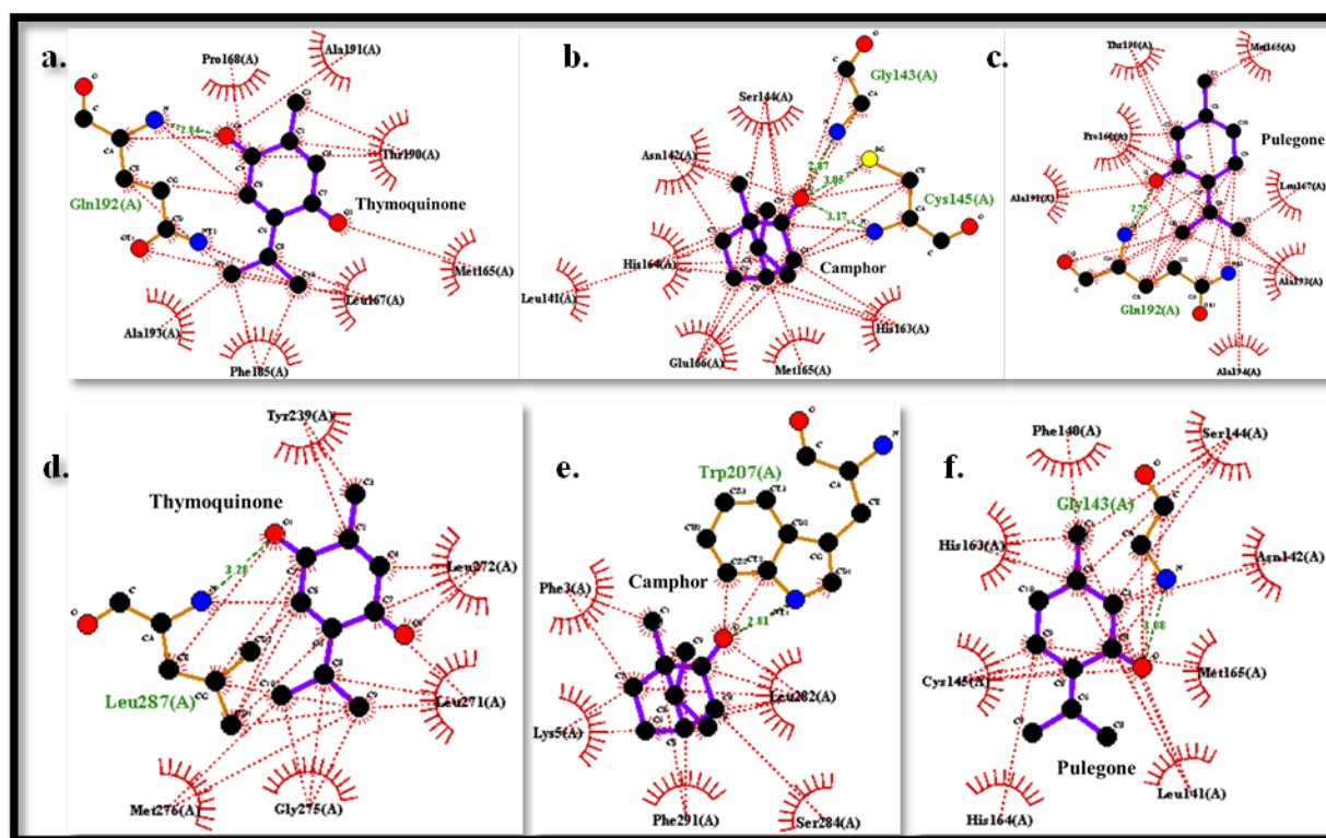
Figure 1. Comparative analysis of interaction between SARS-CoV-2 proteins and natural keto-based natural drugs: (a) 2gtb-Thymoquinone, (b) 2gtb-Camphor, (c) 2gtb-Pulegone, (d) 6lu7-Thymoquinone, (e) 6lu7-Camphor, and (f) 6lu7-pulegone.
