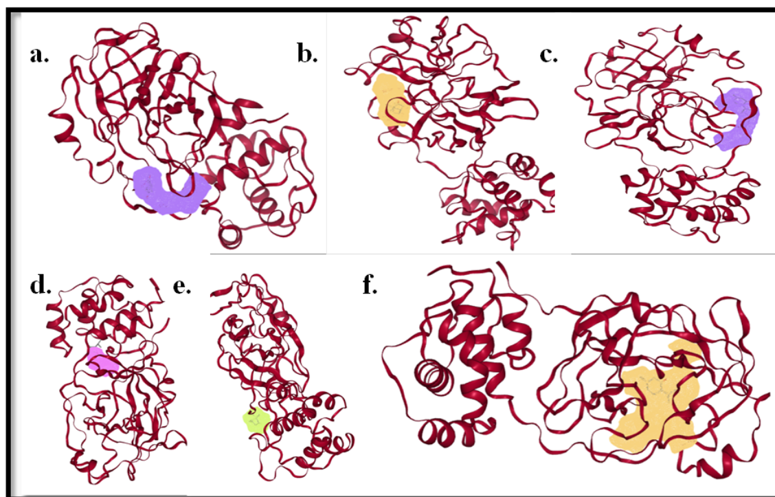
Figure 2. Binding Site for ligands with host protein of SARS-CoV-2: (a) 2gtb-Thymoquinone, (b) 2gtb-Camphor, (c) 2gtb-Pulegone, (d) 6lu7-Thymoquinone, (e) 6lu7-Camphor, and (f) 6lu7-Pulegone.
