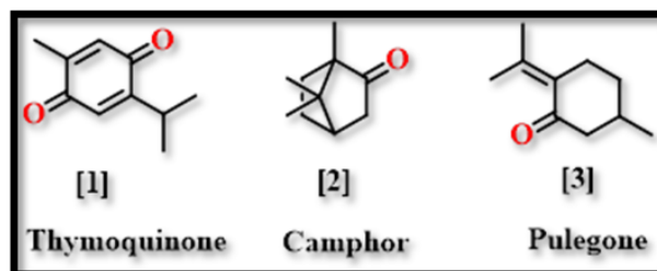
Scheme 1. Chosen keto-based characteristics medication as SARS-CoV-2 objective.
