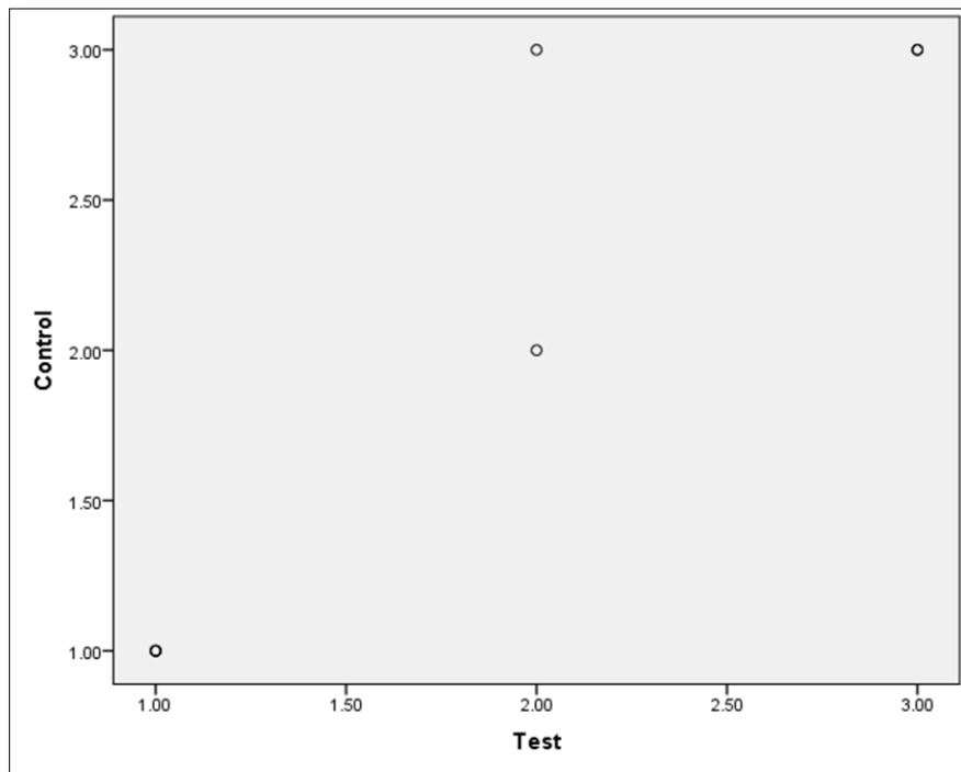
Figure 3. Scatter plot for correlation of mass activity between test and control.
