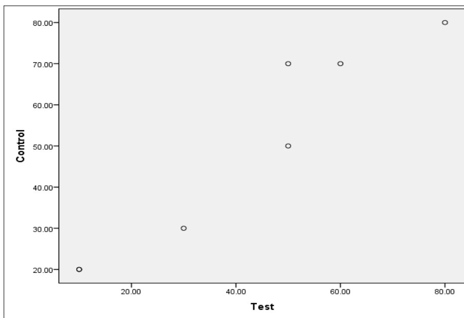
Figure 1. Scatter plot for correlation of motility between test and control.
