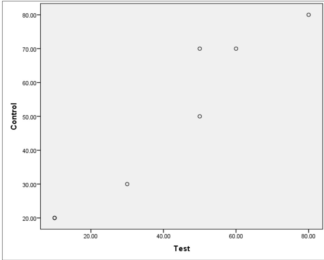
Figure 2. Scatter plot for correlation of percentage live between test and control.
