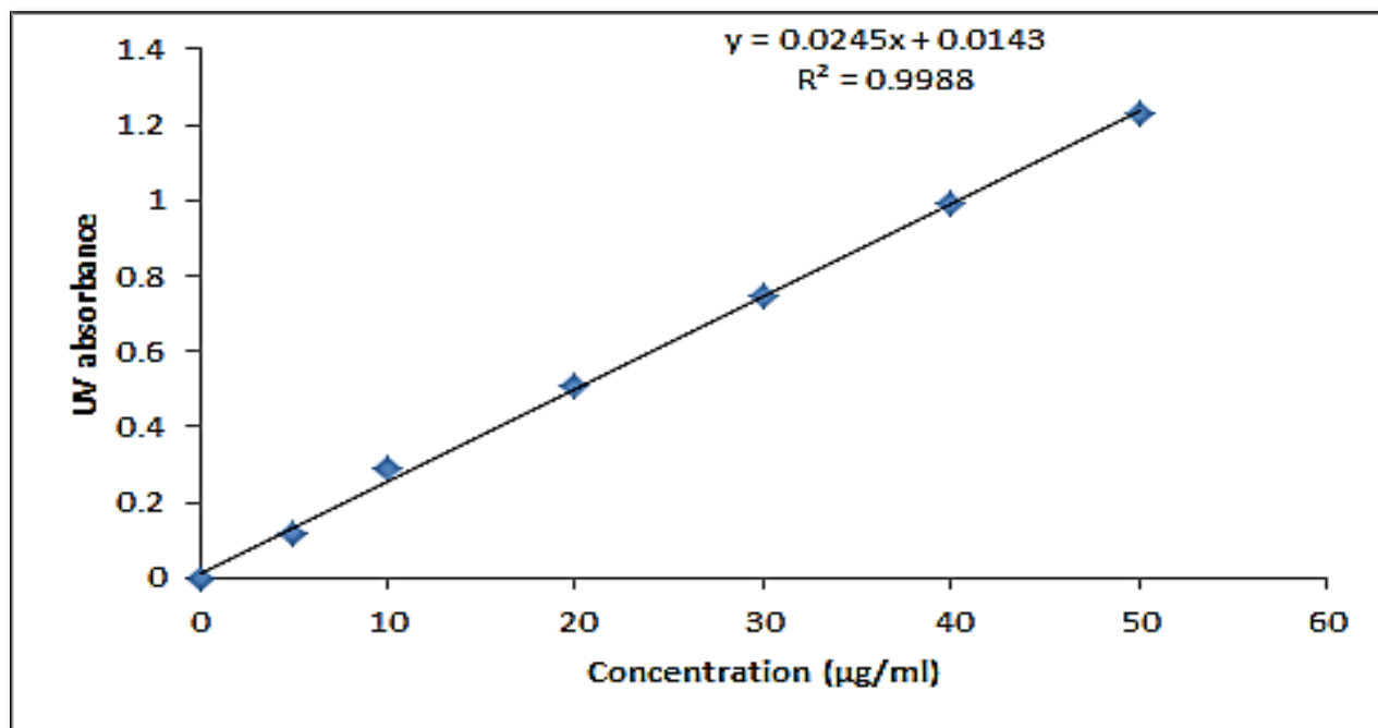
Figure 1. Standard calibration curve of Candesartan Cilexetil in methanol at UV 258 nm.
