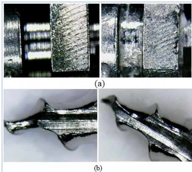
Figure 1. Digital microscopic image showing orthodontic mini-screw implant before insertion (left side) and after removal (right side): a) Head, and b) Tip.
