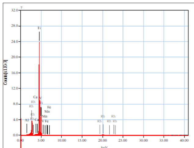
Figure 2. Graphical representation of surface composition of orthodontic mini-screw implants by X-ray fluorescence.
