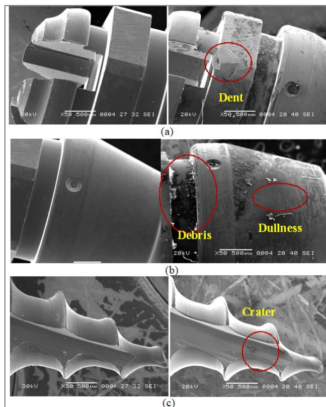
Figure 3. Scanning electron microscopic image showing the morphology and surface changes of MSI before insertion (left side) and after removal (right side): a) Head, b) Collar, and c) Tip.
