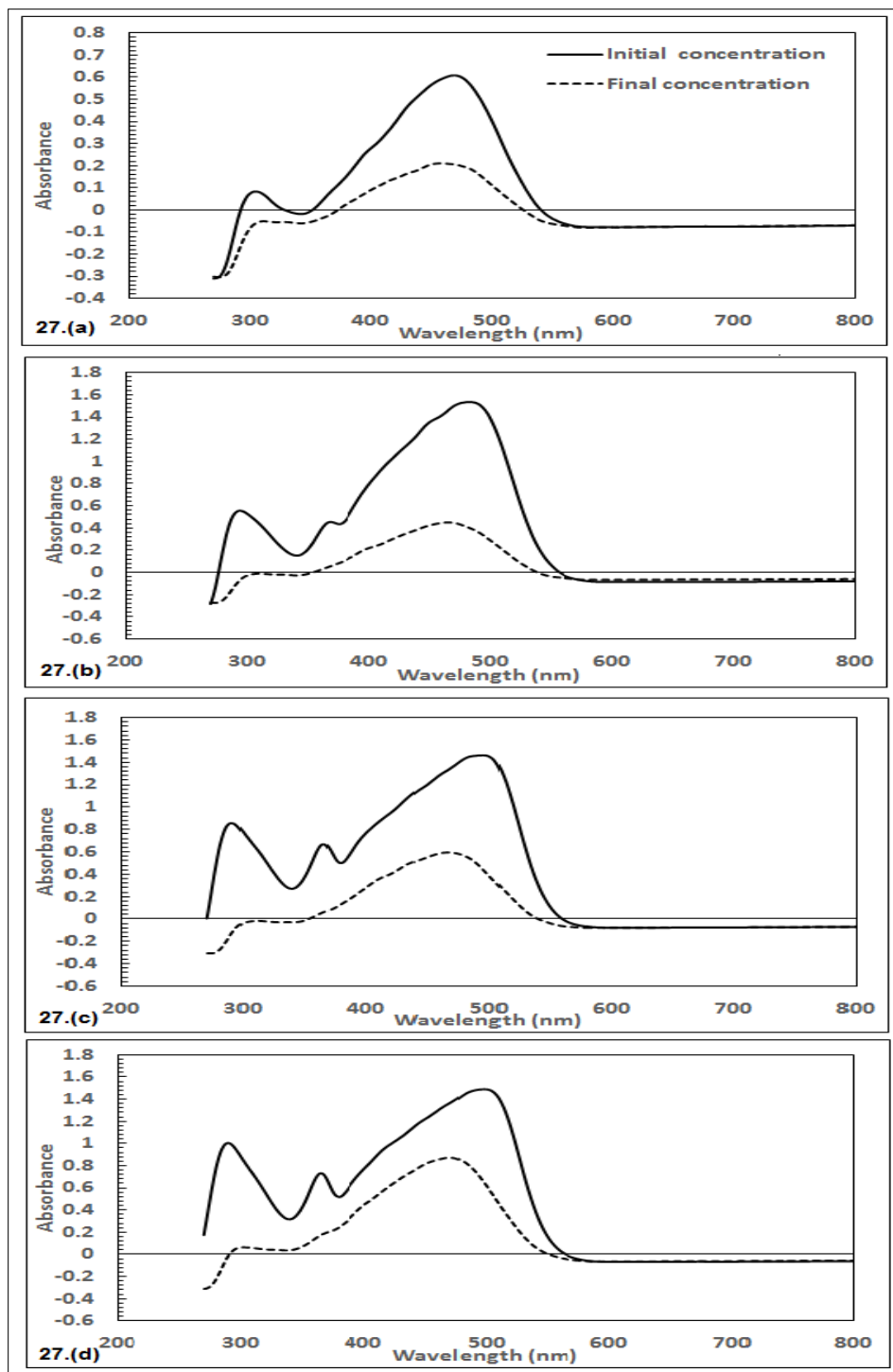
Figure 3. UV-visible spectral profile of culture filtrates before and after biodegradation within 12 days incubation of MO dye concentrations (a) 10 \text{ mg L}^{-1} (b) 30 \text{ mg L}^{-1} (c) 50 \text{ mg L}^{-1} (d) 70 \text{ mg L}^{-1} . Data of these curves represent the mean of three independent measurements.
